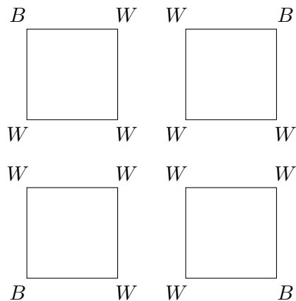
Figure 14.1. Equivalent colorings of square
