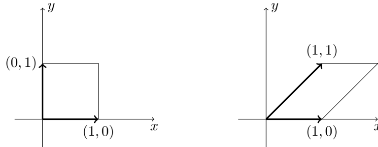
Figure 12.1. SL_2(\mathbb{R}) acting on the unit square
