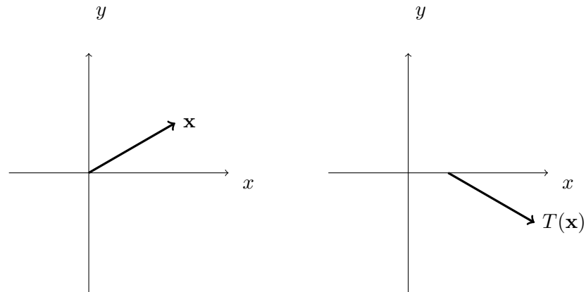
Figure 12.4. Glide reflections
