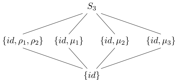
Figure 4.1. Subgroups of S_3
