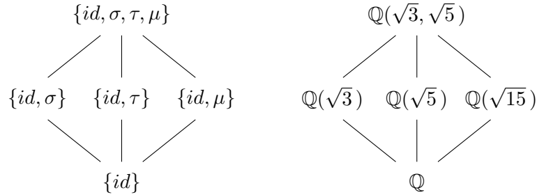
Figure 23.1. G(\mathbb{Q}(\sqrt{3}, \sqrt{5})/\mathbb{Q})
