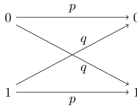
Figure 8.6: Binary symmetric channel
