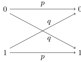
Figure 8.6: Binary symmetric channel
