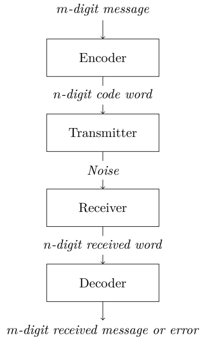
Figure 8.1: Encoding and decoding messages
