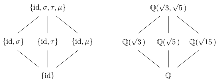
Figure 23.21: G(\mathbb{Q}(\sqrt{3}, \sqrt{5})/\mathbb{Q})
