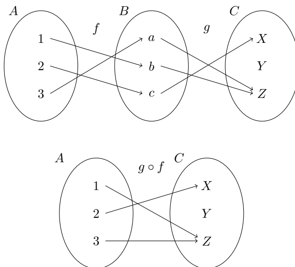
Figure 1.9: Composition of maps
