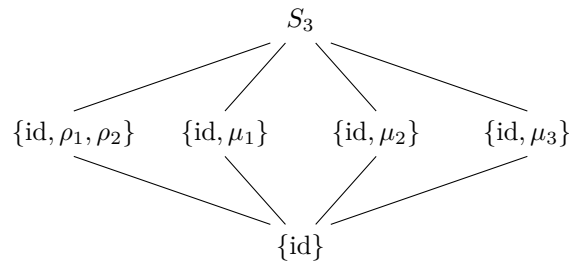
Figure 4.8: Subgroups of S_3
