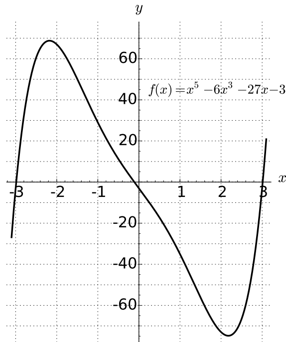
Figure 23.31: The graph of f(x) = x^5 - 6x^3 - 27x - 3
