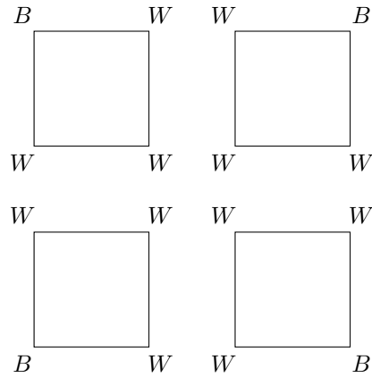
Figure 14.17: Equivalent colorings of square
