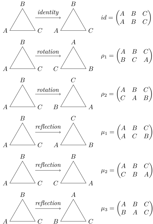
Figure 3.6: Symmetries of a triangle
