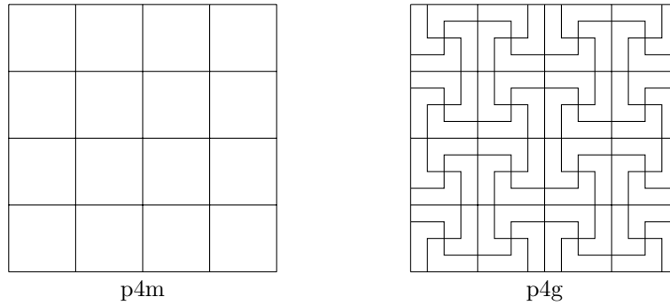
Figure 12.24: The wallpaper groups p4m and p4g
