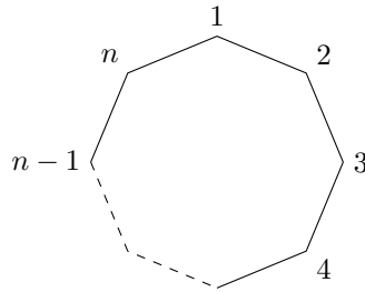
Figure 5.19: A regular n -gon
