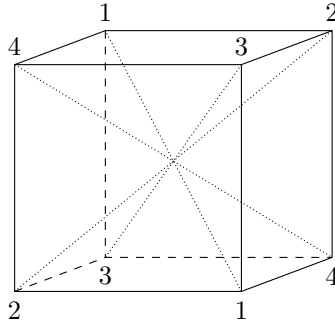
Figure 5.28: The motion group of a cube
