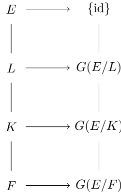
Figure 23.23: Subgroups of G(E/F) and subfields of E
