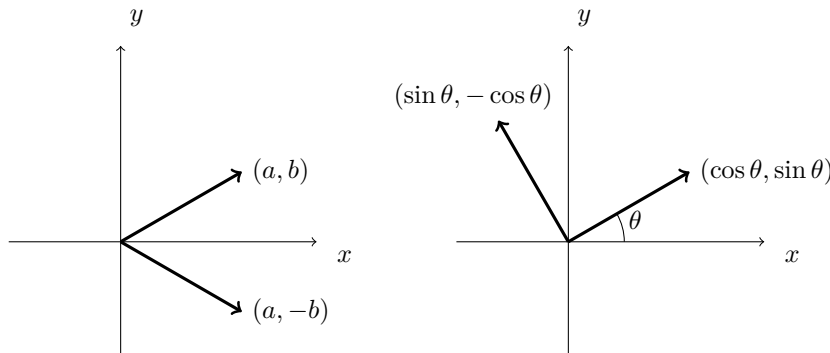
Figure 12.9 O(2) acting on \mathbb{R}^2
