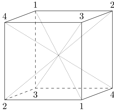
Figure 5.28 The motion group of a cube
