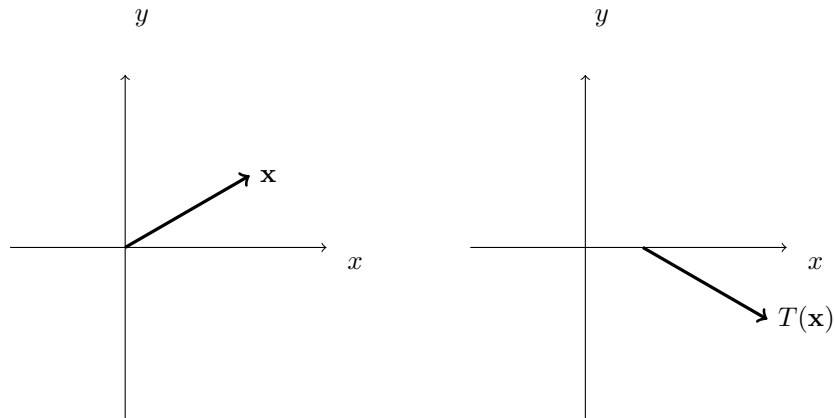
Figure 12.12 Glide reflections
