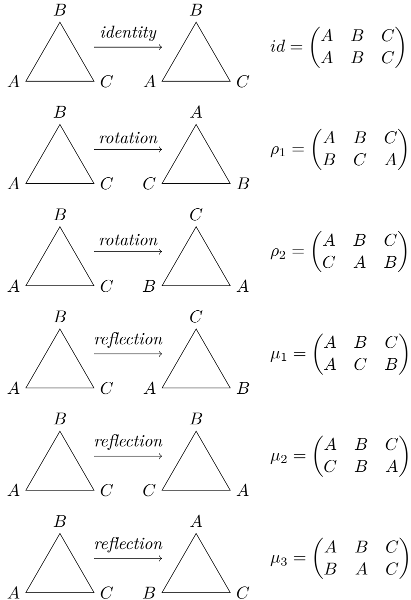
Figure 3.6 Symmetries of a triangle
