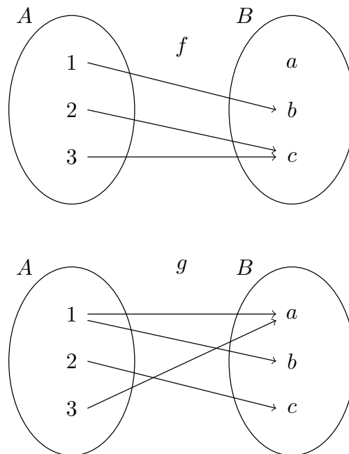
Figure 1.7 Mappings and relations
