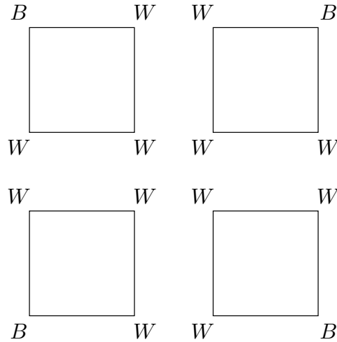
Figure 14.17 Equivalent colorings of square
