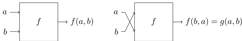
Figure 14.25 A switching function of two variables
