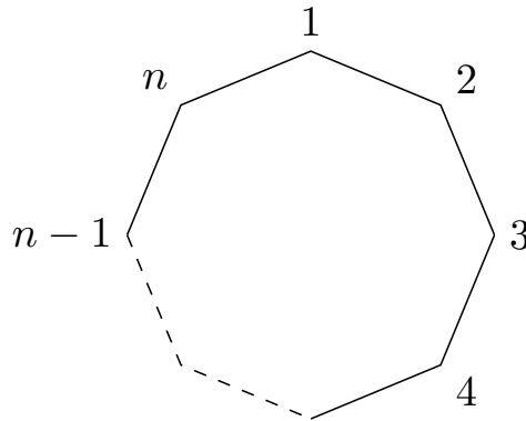
Figure 5.19 A regular n -gon
