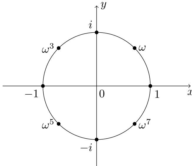
Figure 4.27 8th roots of unity
