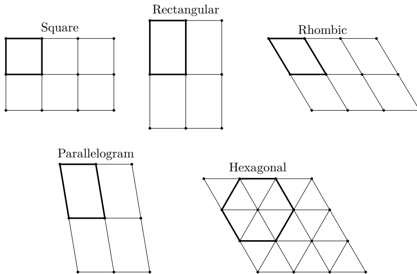
Figure 12.21 Types of lattices in \mathbb{R}^2
