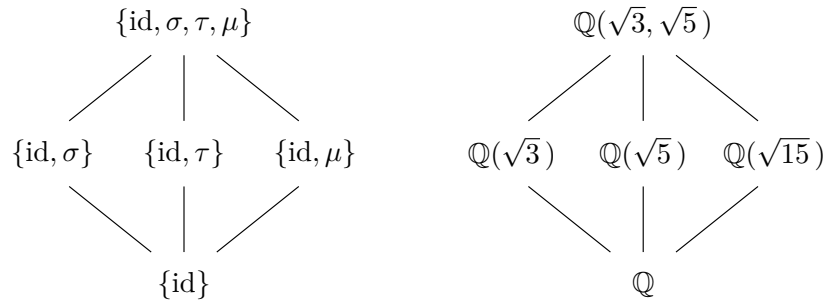
Figure 23.22 G(\mathbb{Q}(\sqrt{3}, \sqrt{5})/\mathbb{Q})
