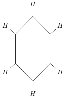
Figure 14.28 A benzene ring
