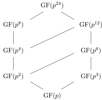
Figure 22.9 Subfields of \text{GF}(p^{24})
