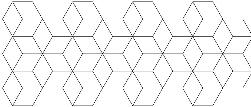
Figure 12.25 Lattice for Exercise 12.4.17, p. 163
