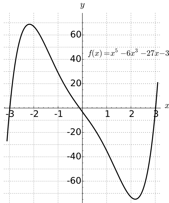
Figure 23.32 The graph of f(x) = x^5 - 6x^3 - 27x - 3
