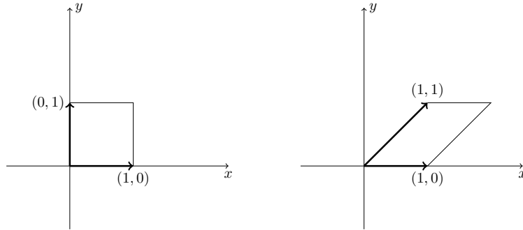
Figure 12.4 SL_2(\mathbb{R}) acting on the unit square
