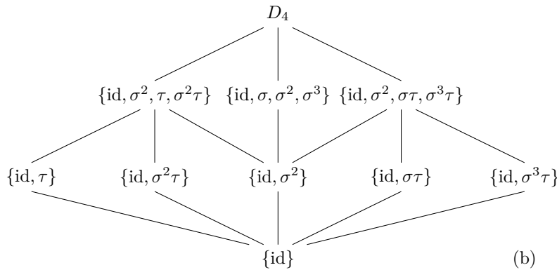
Figure 23.26 Galois group of x^4 - 2
