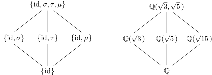
Figure 23.22 G(\mathbb{Q}(\sqrt{3}, \sqrt{5})/\mathbb{Q})
