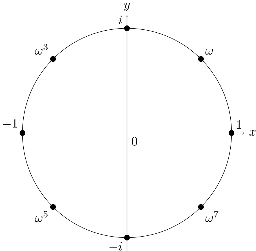
Figure 4.27 8th roots of unity
